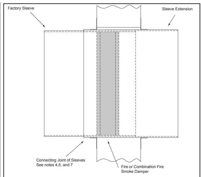
Figure 2: Factory sleeve ends in the plane of the rated barrier.
