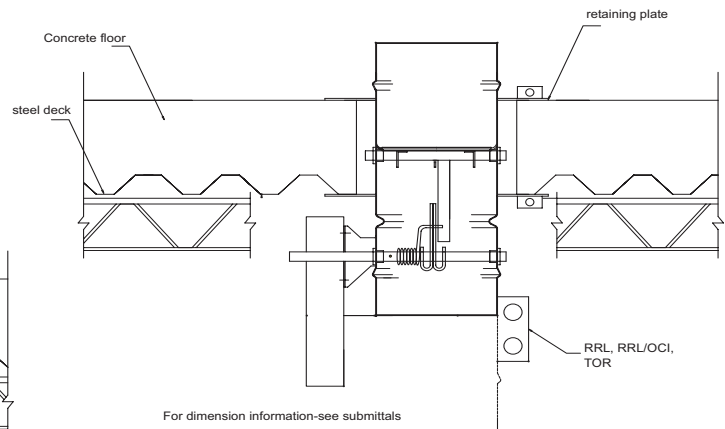
Figure 2: Damper installed in concrete floor with steel deck with actuator below the floor.
