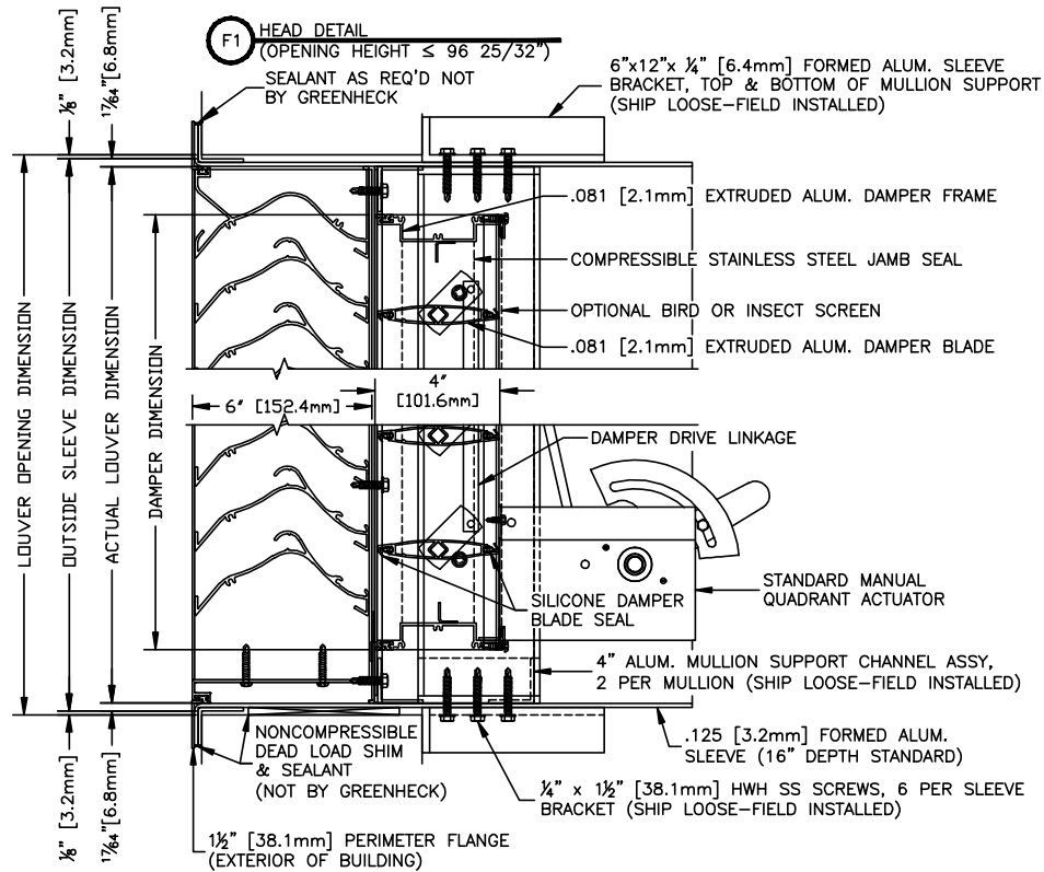
G1 SILL DETAIL (OPENING HEIGHT \leq 96 \frac{25}{32} ")
