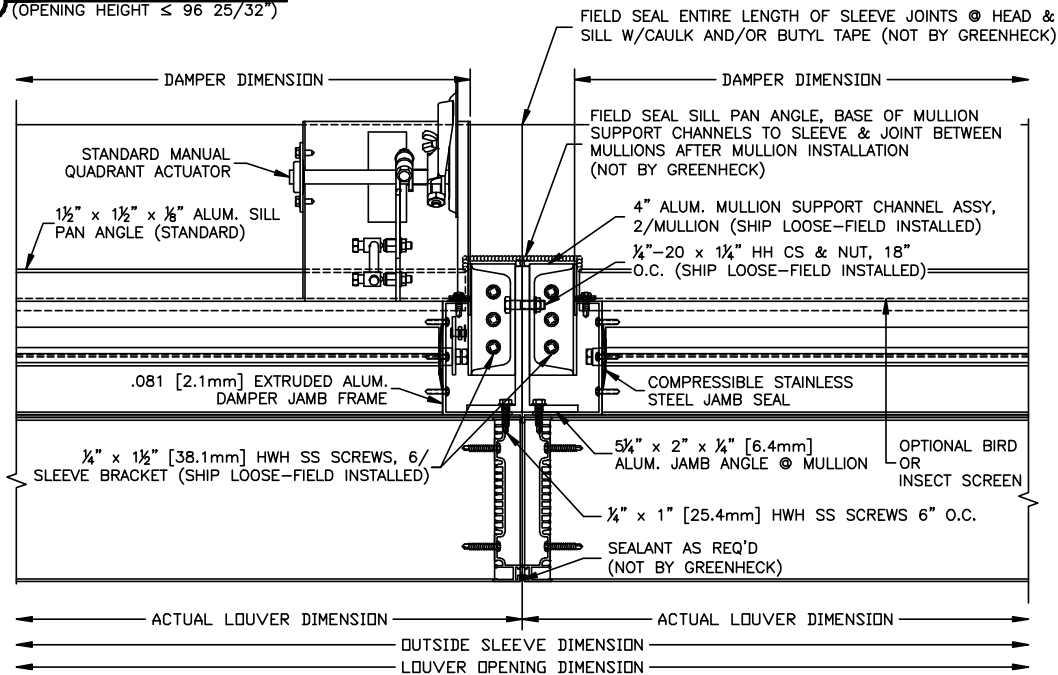
H1 MULLION DETAIL (OPENING HEIGHT \leq 96 \frac{25}{32} ")
