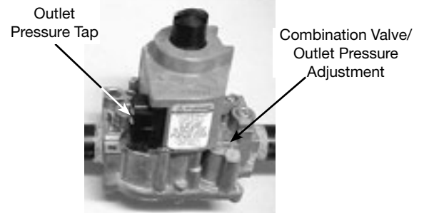
Combined Regulator Valve
