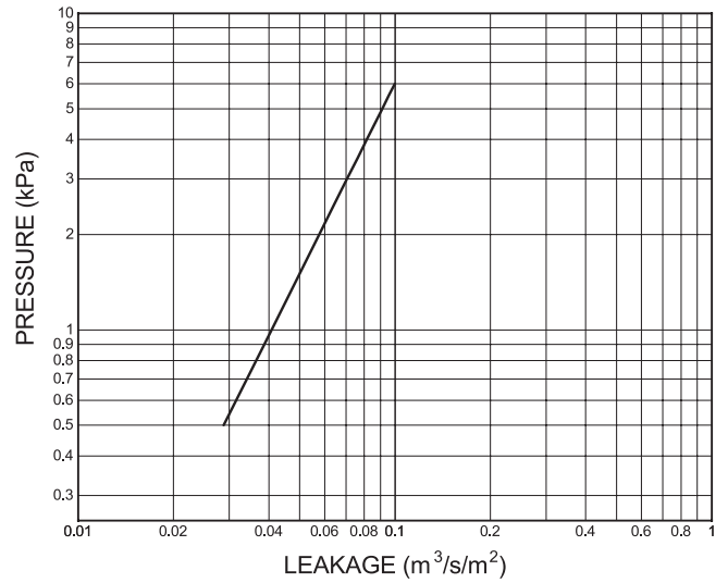
Leakage (metric version)
