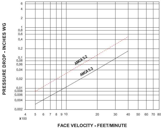
Pressure Drop (english version) 42 in. x 42 in. (1067mm x 1067mm) Damper
