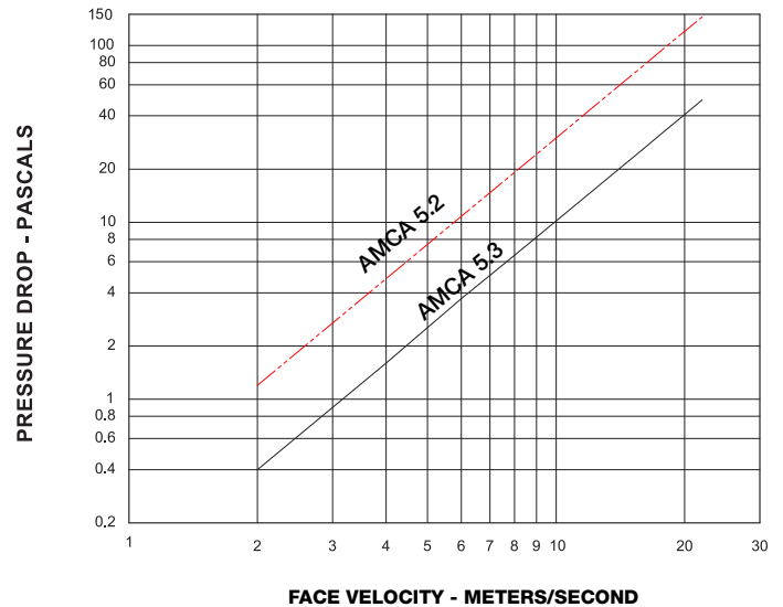
Pressure Drop (metric version) 42 in. x 42 in. (1067mm x 1067mm) Damper
