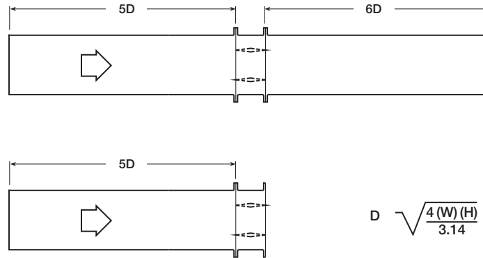
Pressure Drop (english version) 42 in. x 42 in. (1067mm x 1067mm) Damper
