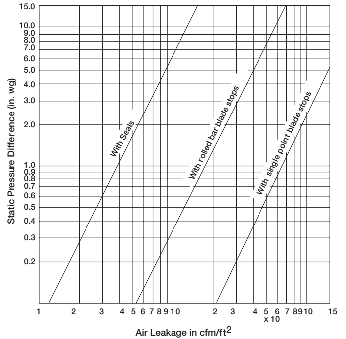
36 in. Diameter Damper
