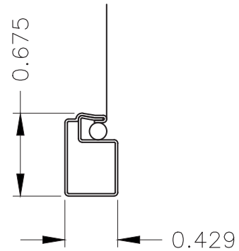
SCREEN FRAME DETAIL
