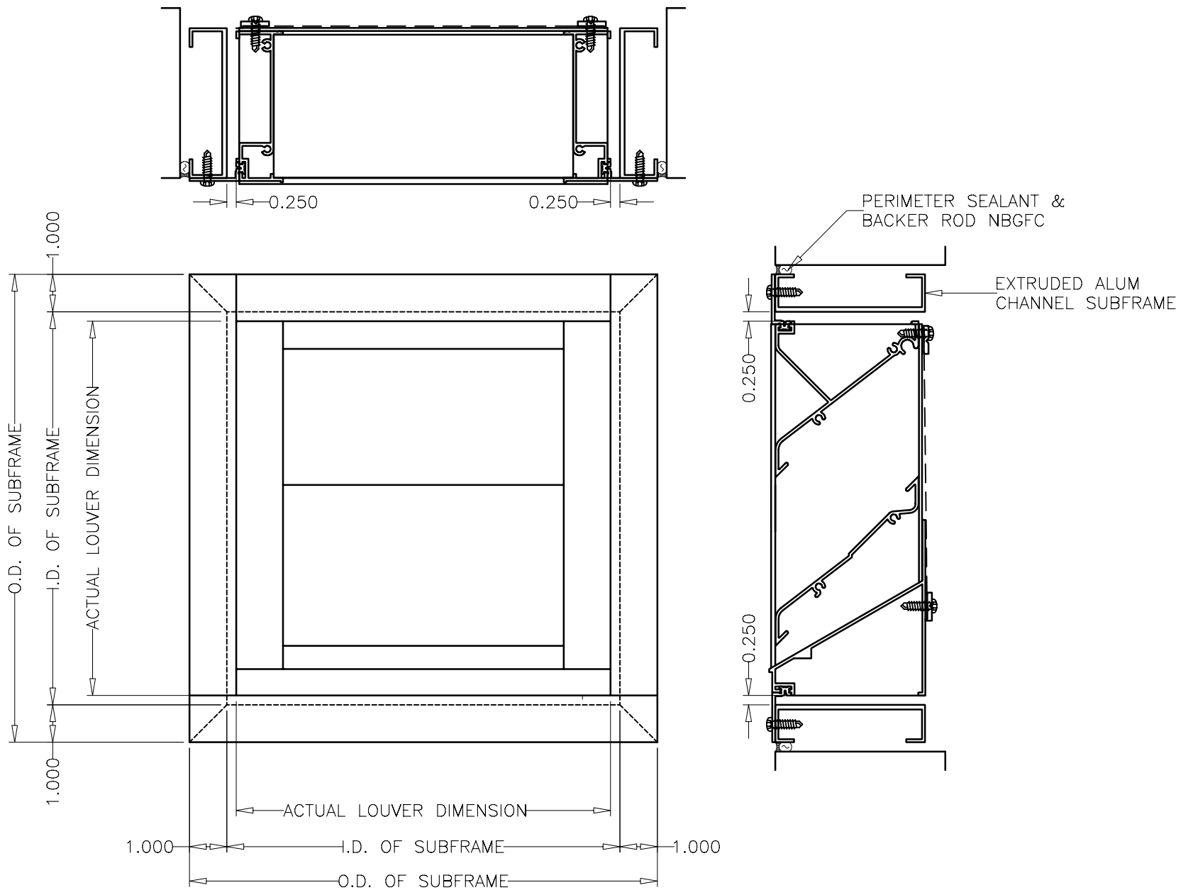
STANDARD GREENHECK SUBFRAME DETAIL
