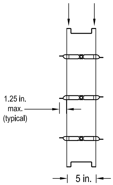
Standard Flange Frame
