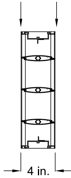
Standard Frame
