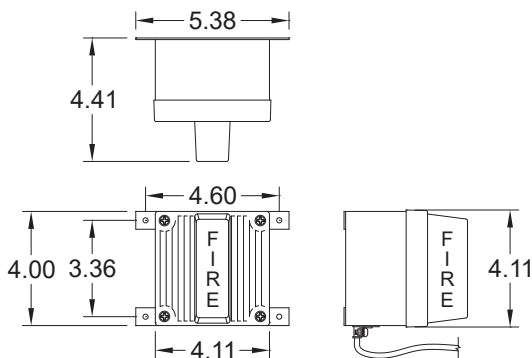
Dimensions shown are in inches.
