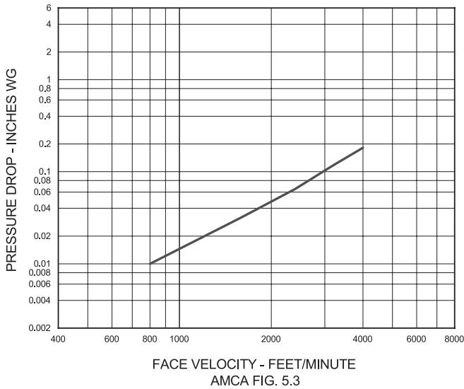
Pressure Drop (english version) 42 in. x 42 in. (1067mm x 1067mm) Damper
