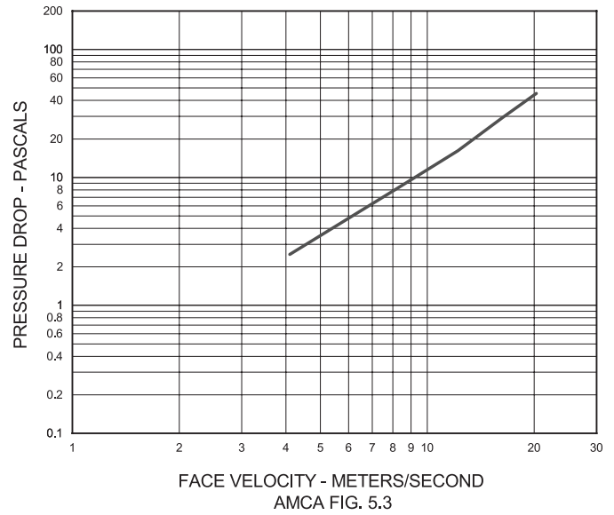
Pressure Drop (metric version) 42 in. x 42 in. (1067mm x 1067mm) Damper
