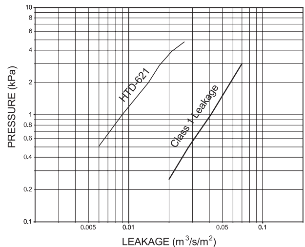
Leakage (metric version) 42 in. x 42 in. (1067mm x 1067mm) Damper
