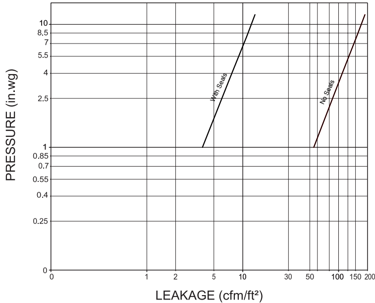
20 x 20 in. (508mm x 508mm) Damper
