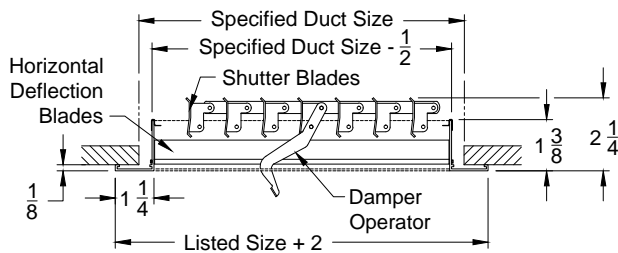
Model: XG-H4002M-1 Single Deflection Register Multi-Shutter Damper - Horizontal Front Blades
