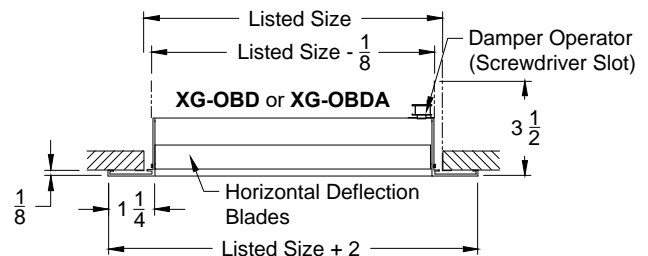
Model: XG-H4002-1 Single Deflection Register - Horizontal Blades with Opposed Blade Damper
