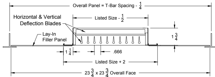
Model: XG-V4004S-6 (Double Deflection Grille) Lay in T-Bar - With Filler Panel (Vertical Front Blades)
