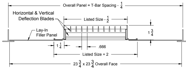
Model: XG-H4004S-6 (Double Deflection Grille) Lay in T-Bar - With Filler Panel (Horizontal Front Blades)
