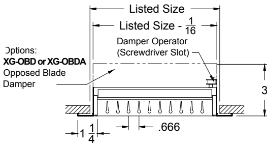
Option: XG-V4004S-1 XG-OBD ( Double Deflection Register ) ( Vertical Front Blades ) With Opposed Blade Damper
