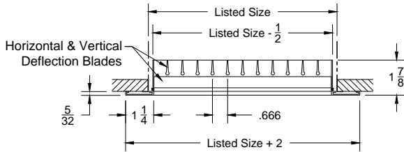
Model: XG-H4004-1 (Double Deflection Grille)(Horizontal Front Blades)
