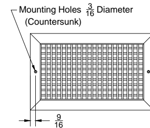
Face View (Double Deflection) (Vertical Front Blades)
