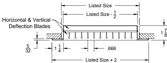
Model: XG-V4004-1 (Double Deflection Grille) (Vertical Front Blades)
