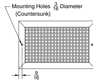
Face View (Double Deflection) (Horizontal Front Blades)
