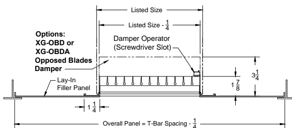
Model: XG-H4004-6 (Double Deflection Grille) Lay in T-Bar - With Filler Panel (With Damper - Horizontal Front Blades)
