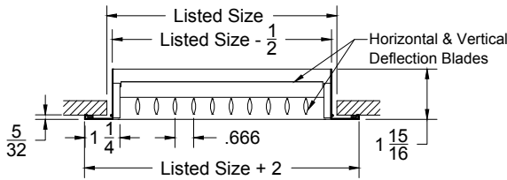
Model: XG-H4004-AF-1 XG-OBD ( Double Deflection Register ) ( Horizontal Front Blades ) With Opposed Blade Damper
