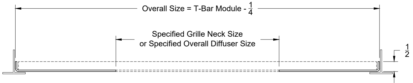
Side View
