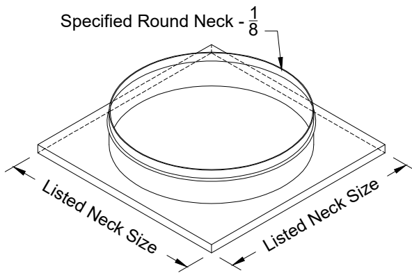
Iso View
