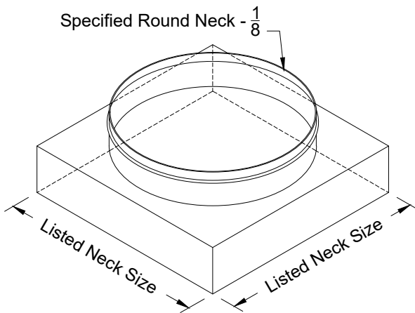
Iso View
