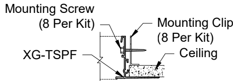
Optional XG-TSPF Mounting Kit - TBPFMK
