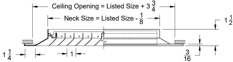
Side View
