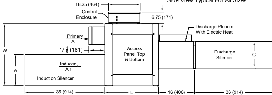
Top View Typical For Case Sizes 2 - 5
