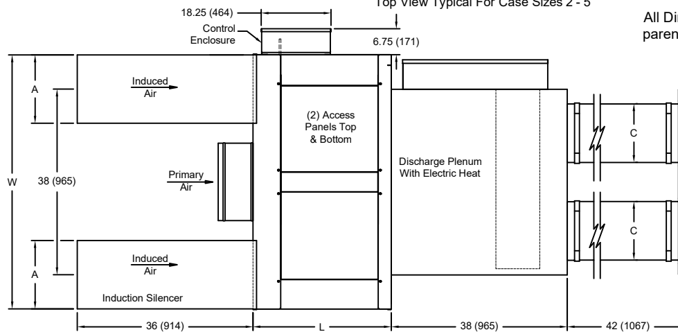
Top View Typical For Case Sizes 6&7
