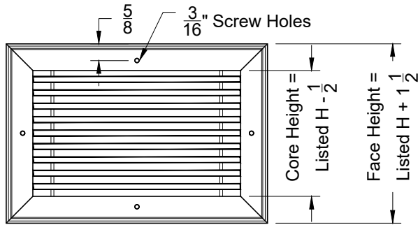
Face View
