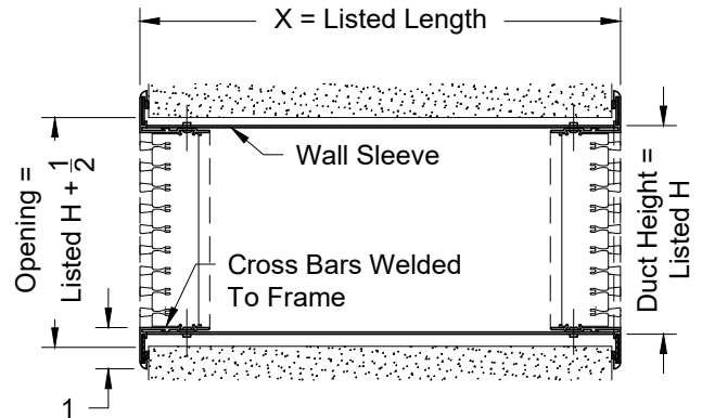
End View
