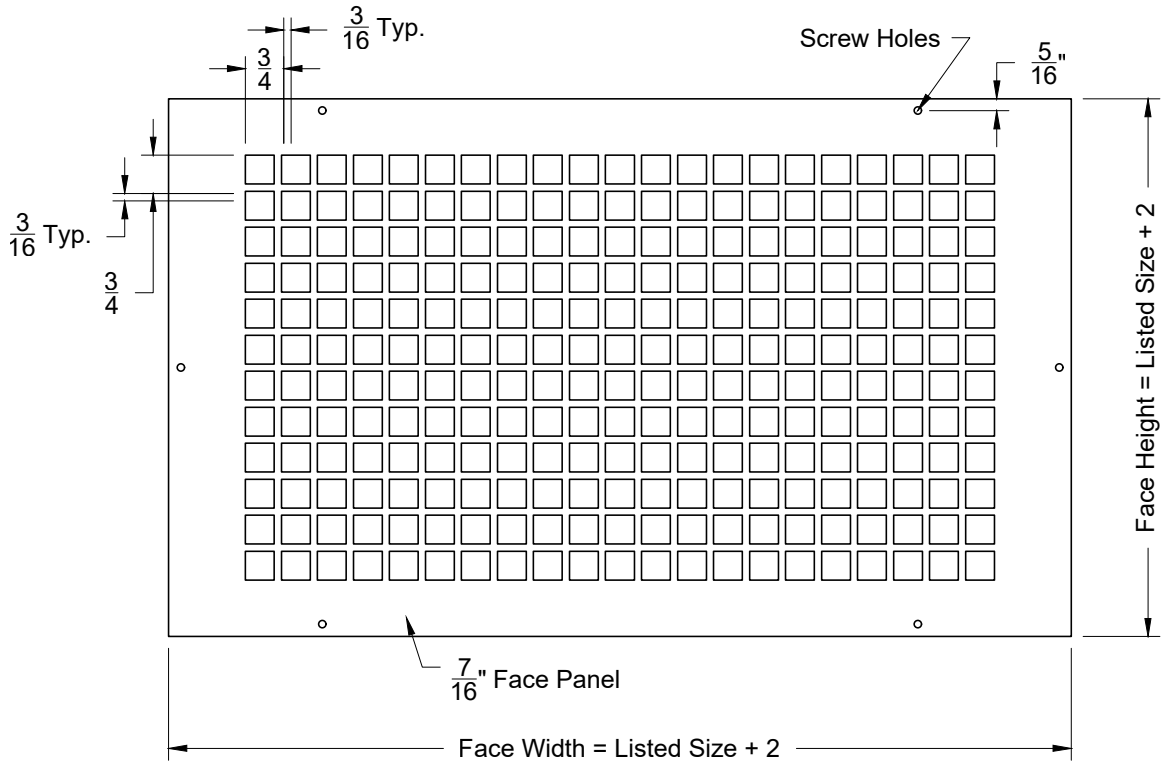
Face View
