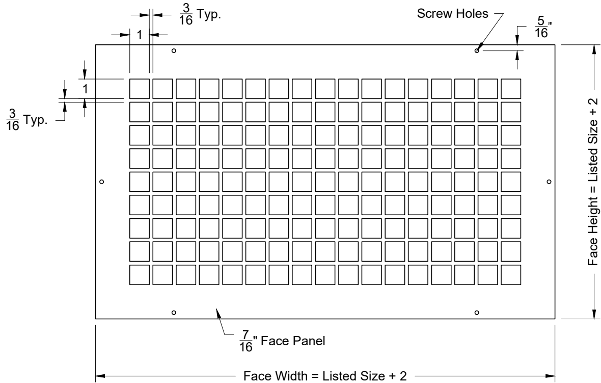
Face View
