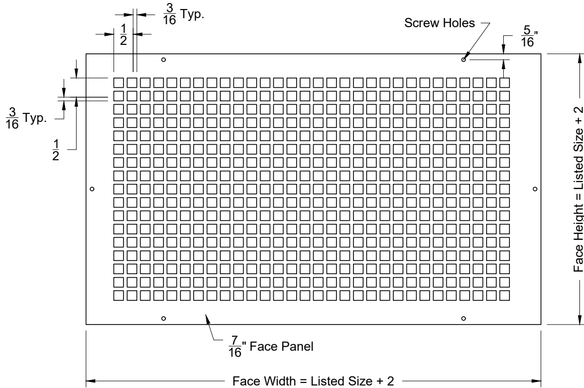
Face View
