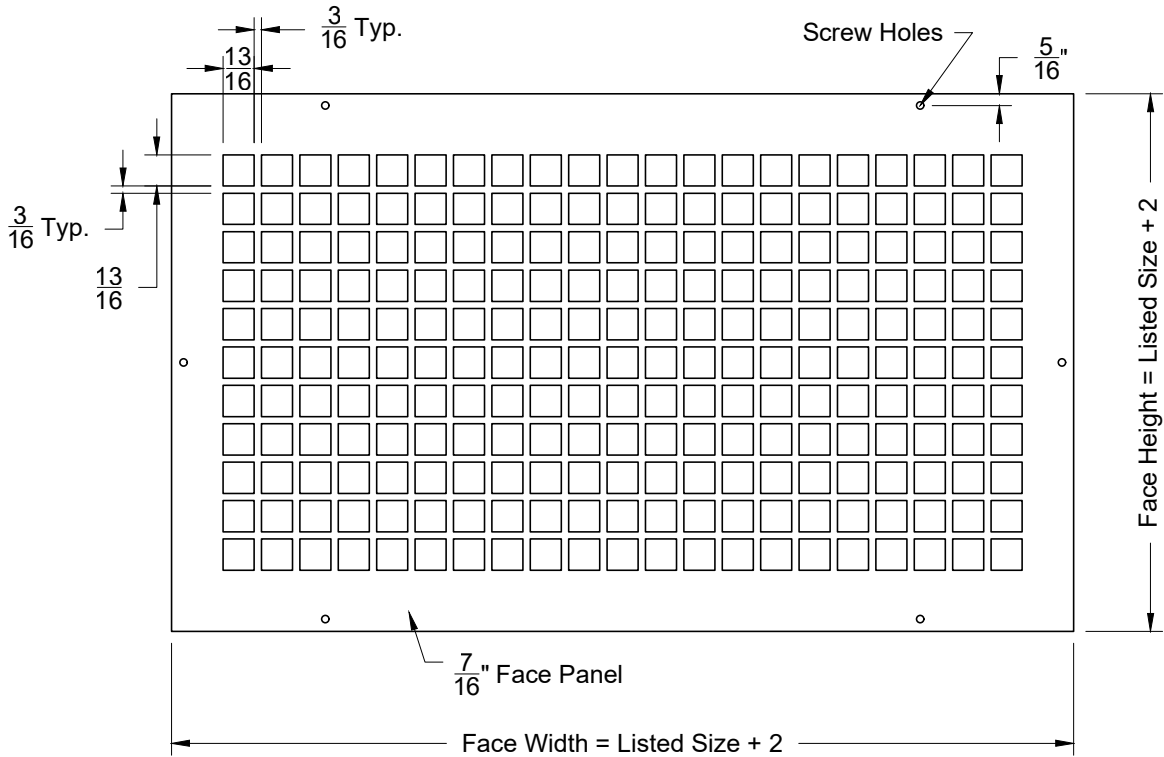
Face View
