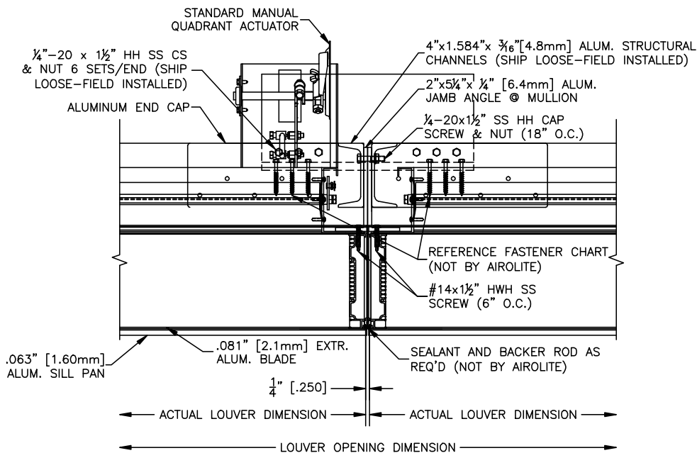
H2 MULLION DETAIL (OPENING HEIGHT \leq 96 \frac{1}{2} )
