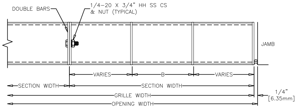
VERTICAL MULLION
