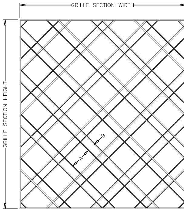
EXTERIOR ELEVATION
