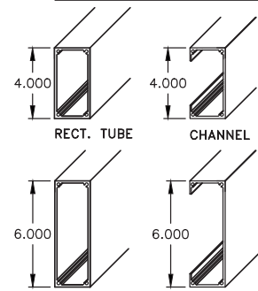
OPTIONAL FASCIA OUTRIGGER STYLE WILL VARY
