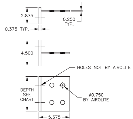
OPTIONAL MOUNTING BRACKETS
