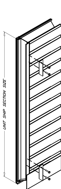
SINGLE SECTION ANCHOR CLIPS INSTALLATION
