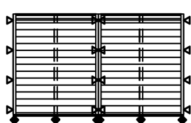
MULTIPLE SECTIONS WIDE, SINGLE SECTION HIGH (SUPPORTED MULLION)
