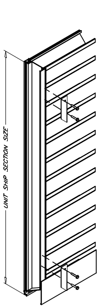
SINGLE SECTION ANCHOR CLIPS INSTALLATION
