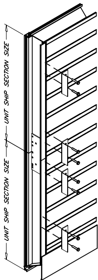
MULTIPLE SECTION HIGH ANCHOR CLIPS INSTALLATION
