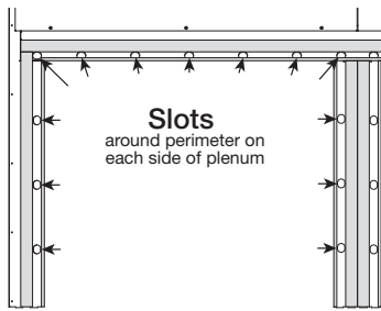
Slot Detail
