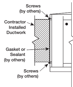
Exterior connection All Sizes
