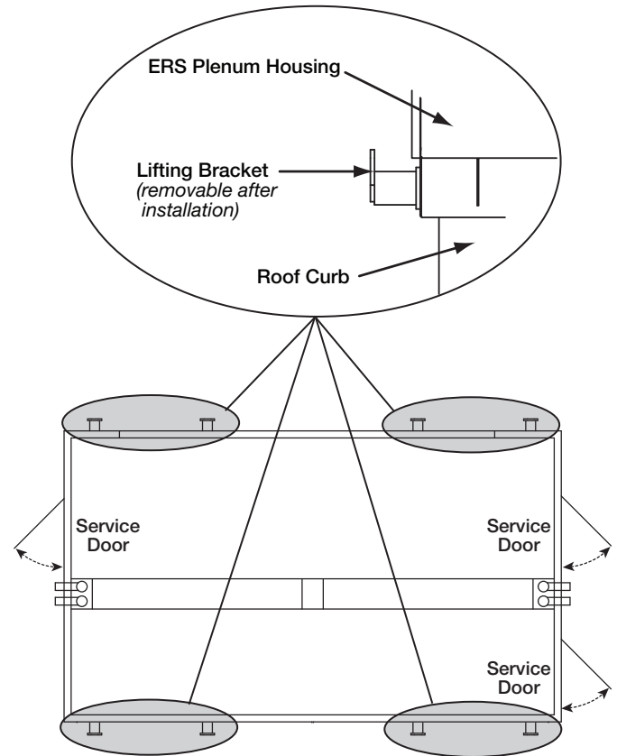
Top View of ERS Plenum Section
