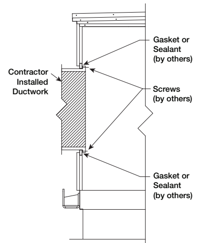
Interior flanged ductwork connection ERS 20-65
