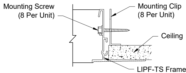
LIPF-TS - Mounting Detail TBPFMK Mounting Kit
