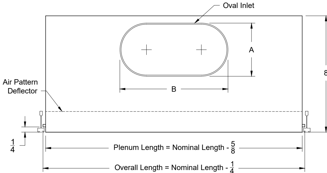
Front View
