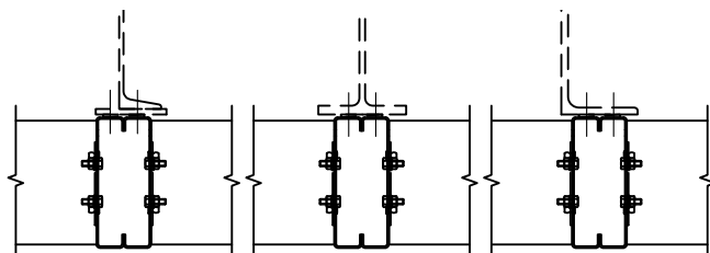
ALTERNATE MULLION STRUCTURAL SUPPORT EXAMPLES
