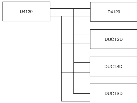
FIGURE 8. MULTIPLE FAN SHUTDOWN (INTERCONNECTION OF DUCTSD TO D4120):
