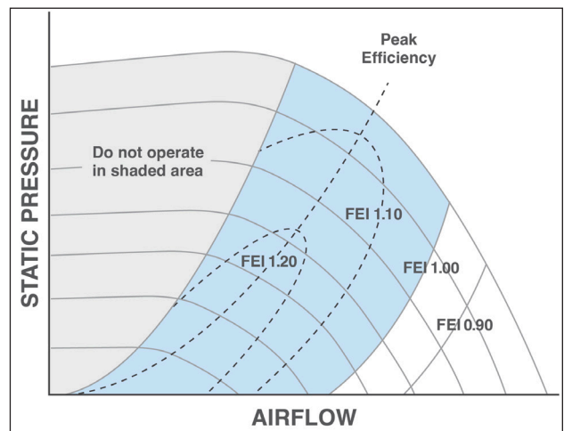
Figure 3. FEI values for different operating regimes defined by airflow and static pressure for a fan controlled by a VFD. The blue shaded area shows where the fan is compliant if the minimum FEI value is set at 1.00.
