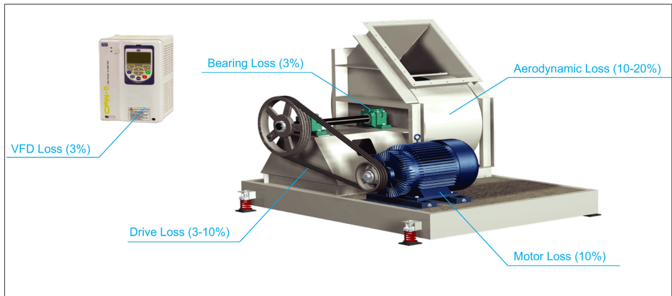
Figure 1. Elements of a wire-to-air measurement of a fan system.
