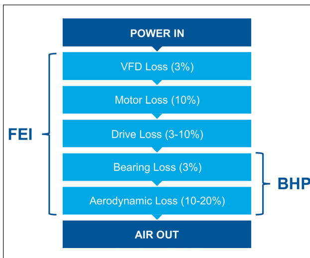
Figure 2. Wire-to-Air losses in a fan with approximate “normal” losses for each component. Note that brake horsepower only accounts for 13–23% of losses.
