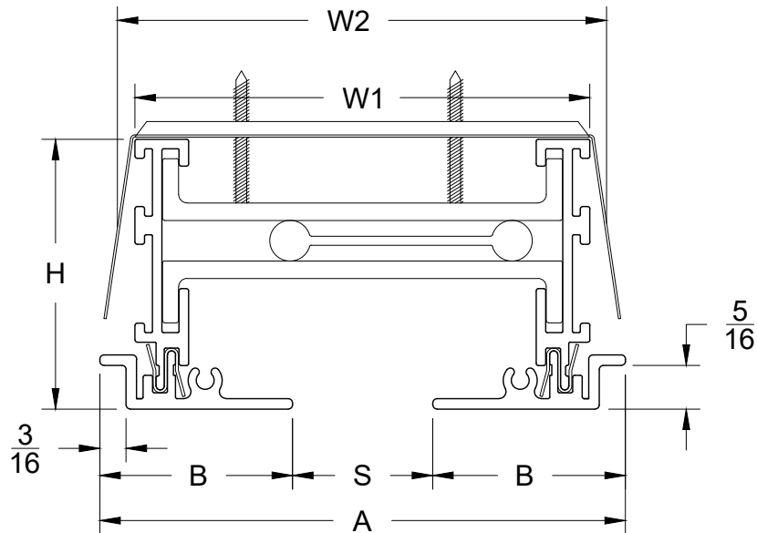
Section View
