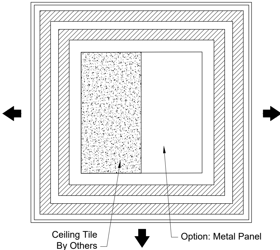
Face View
