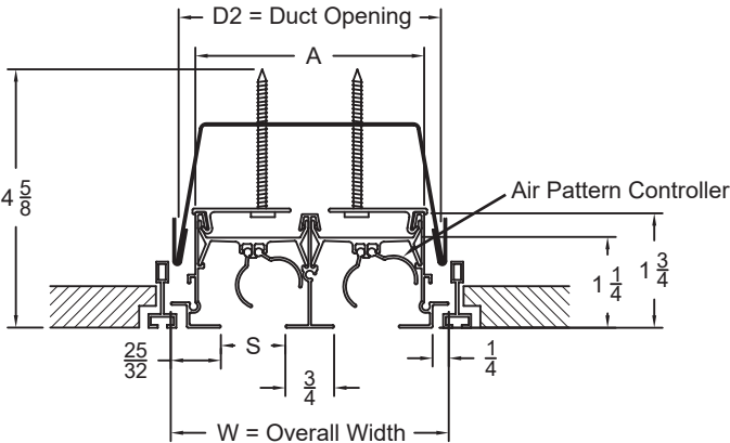
LSD-DD-9 Concealed Mount (With Hardware)
