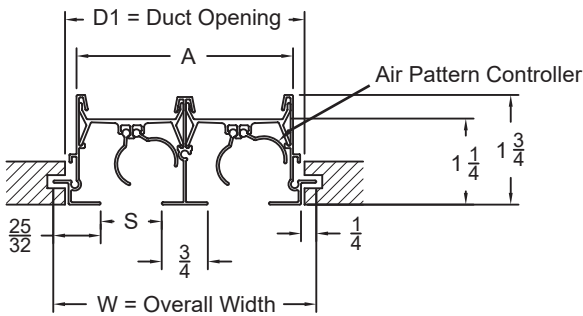
LSD-DD-7 Standard Mount (No Hardware)
