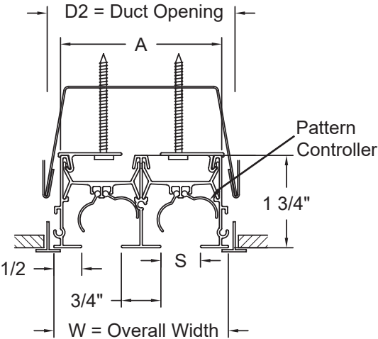
LSD-FF-6 Concealed Mount (With Hardware)
