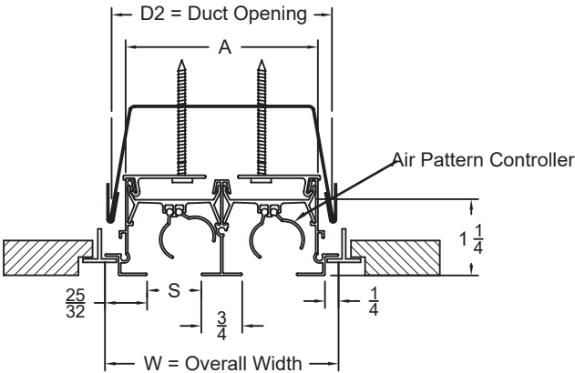
LSD-DD-8 Concealed Mount (With Hardware)
