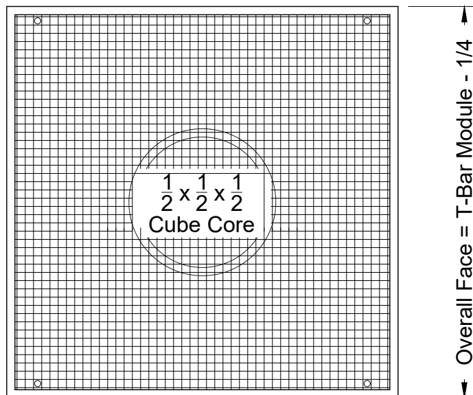
Face View
