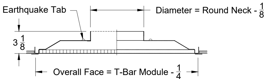
Side View
