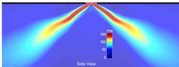
Isothermal (2 Way Throw Pattern Shown)
