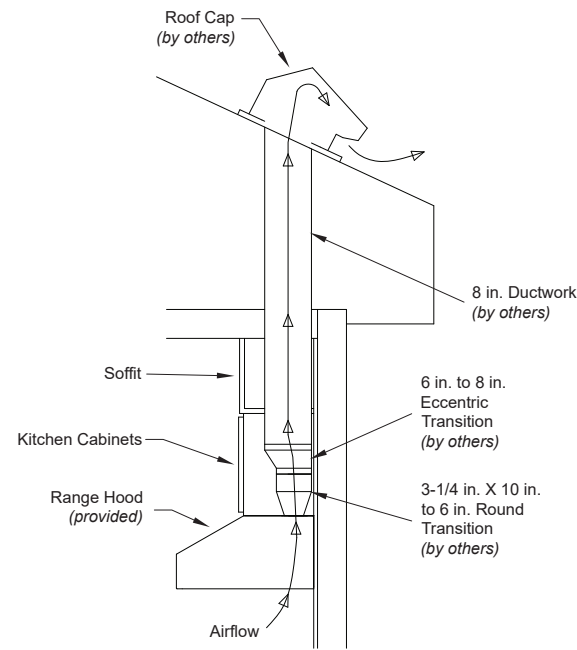
Integral Fan | Top Discharge 8" Round Duct
